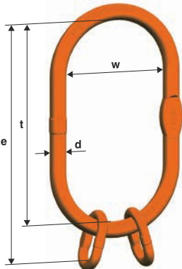
VLW 2/4 Oversize master link assembly
