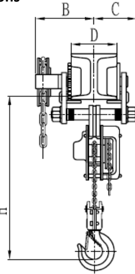
3.0t twin fall
