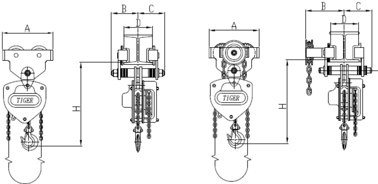
0.5t – 2.0t & 3.0t single bar plain trolley
