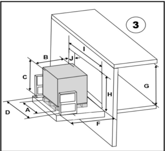
3. Loading onto a balcony with an opening or doorway
