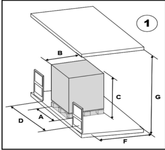
1. Loading by forklift to a mezzanine or platform
