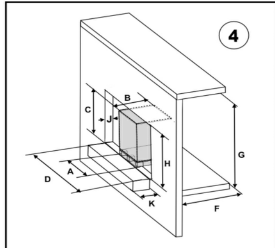
4. Loading through an opening or doorway, If the opening has a runway beam (See fig.2) tell us the height to underside of beam E.
