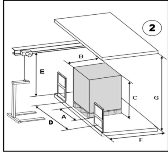
2. Loading by hoist to a mezzanine or platform
